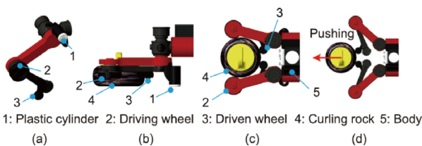
Fig. 6. The multiple functions of the front legs. (a) The virtual prototype of front leg; (b) the front and (c) top view; and (d) the front legs are pushing the curling rock.
