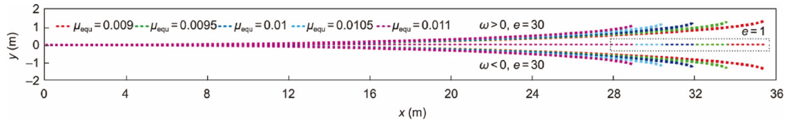
Fig. 14. Calculated trajectories of the curling rock with different ratios e and equivalent friction coefficients \mu_{equ} .
