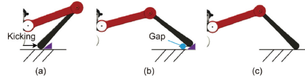
Fig. 8. The multiple functions of the rear legs. (a) the beginning and (b) ending positions of rear leg during kicking the hack; (c) the rear leg is decreasing the forward velocity by friction force.
