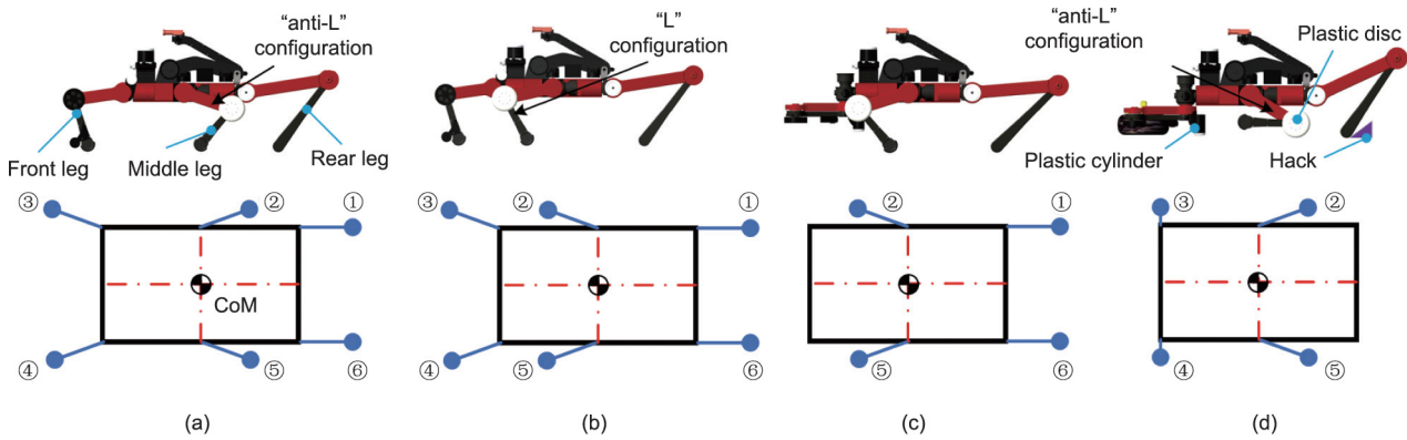
Fig. 4. The morphology transformation of the robot legs between different tasks. All legs are supporting the body and the middle legs are (a) “anti-L” configuration while (b) “L” configuration. (c) The middle and rear legs are supporting the body and the front legs are preparing for gripping rock; (d) the plastic cylinders and discs are supporting the body.
