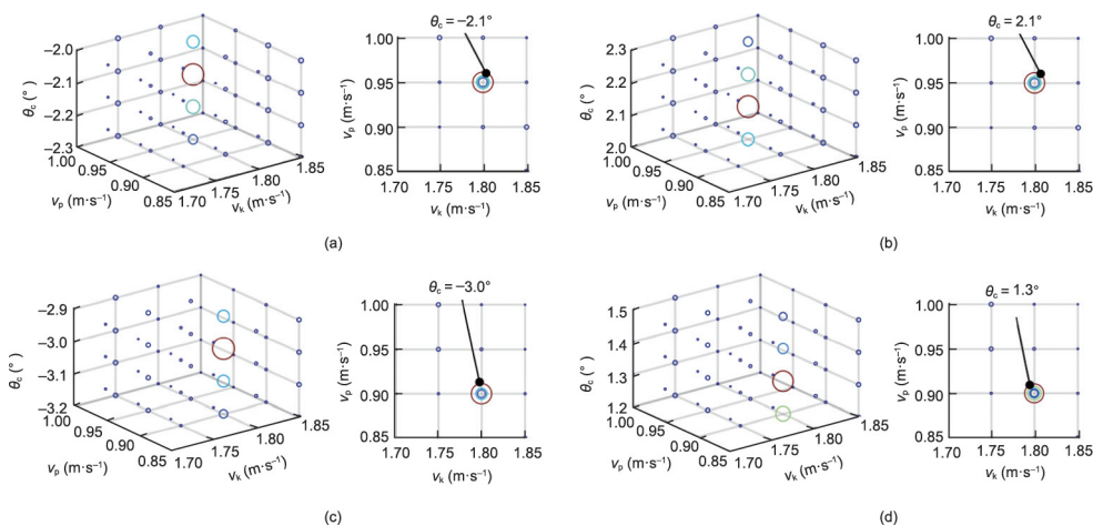
Fig. 17. Searching results for optimal parameters with fixed intervals. (a) Anticlockwise and (b) clockwise curling rocks towards the center of the house, while (c) anticlockwise and (d) clockwise curling rocks towards a general targeted point.
