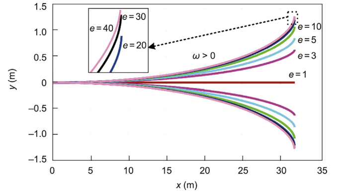
Fig. 13. The calculated trajectory of the curling phenomenon under different ratios e and rotation directions.
