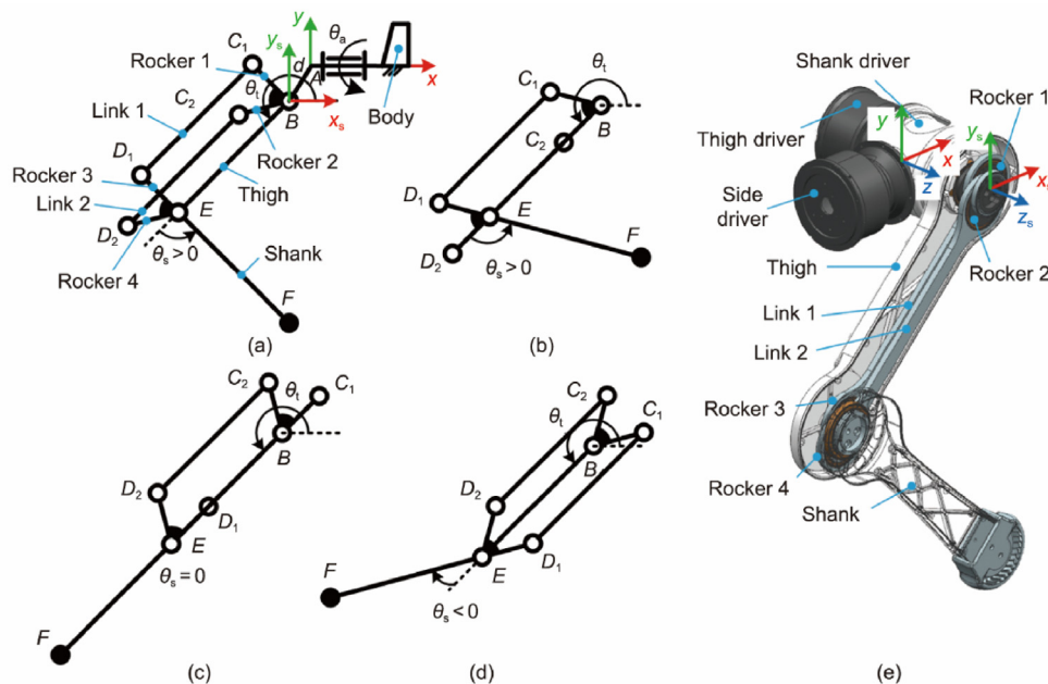
Fig. 5. The configuration switching principle of the leg mechanism. (a) The schematic diagram of mechanism of single leg; (b) the leg is “L” configuration, (c) the critical switch state or (d) “anti-L” configuration; (e) the virtual prototype.
