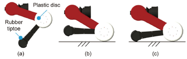
Fig. 7. The multiple functions of the middle legs. (a) The virtual prototype of middle leg; (b) the plastic disc is supporting the body and (c) the middle leg is decreasing the forward velocity by friction force.
