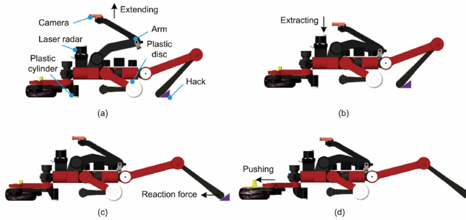
Fig. 3. The robot's movements when throwing a curling rock. (a) The extending and (b) extracting process of the carried arm. (c) The rear legs are kicking the hack to obtain the forward reaction force. (d) The front legs are pushing the curling rock to speed up again.
