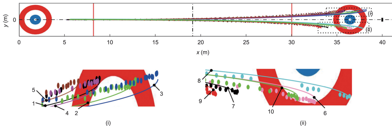
Fig. 16. Calculated trajectories (solid line) and measured trajectories (dotted line) of the curling rock with \theta_c = 0^\circ . (i) The left below and (ii) the right below figures are the terminal trajectories of clockwise and anticlockwise rocks.
